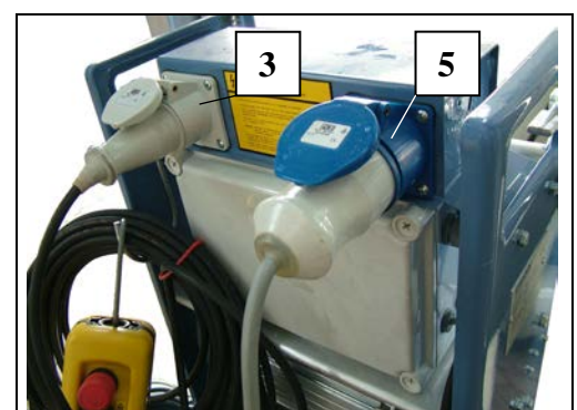
Fig. 7 Winde FIXLIFT 250
